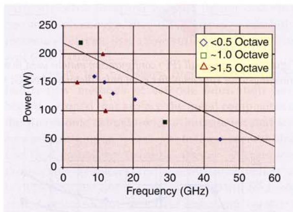
Figure 7. Average output power of sample microwave power modules (MPMs). The diamonds are MPMs with less than 0.5 octave bandwidth; the squares are MPMs with one octave bandwidth; the triangles are MPMs with greater than 1.5 octave bandwidth.
