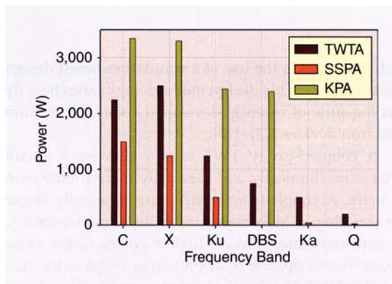
Figure 5. Typical power of commercial satellite communication high-power amplifiers including traveling-wave tube amplifier (TWTA), klystron power amplifier (KPA) and solid-state power amplifier (SSPA).
