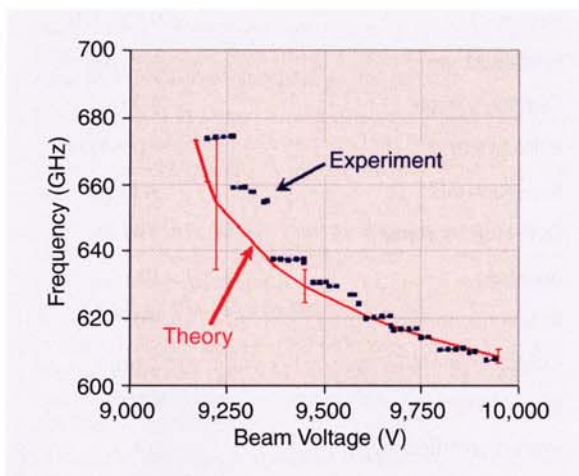
Figure 20. Terahertz source operating frequencies.
