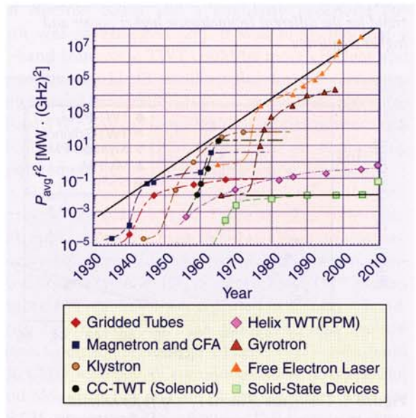
Figure 2. Seven decades of progress in Pf^2 for various power amplifier types.
