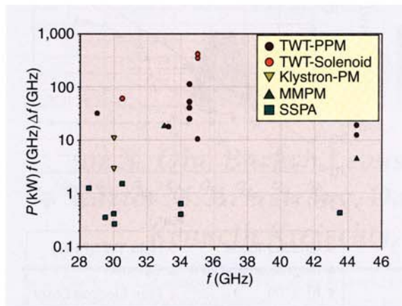
Figure 4. The figure of merit Pf^2(\Delta f/f) for selected millimeter-wave power amplifiers including traveling-wave tube (TWT) amplifier, millimeter-wave power module (MMPM), klystron, and solid-state power amplifier (SSPA).
